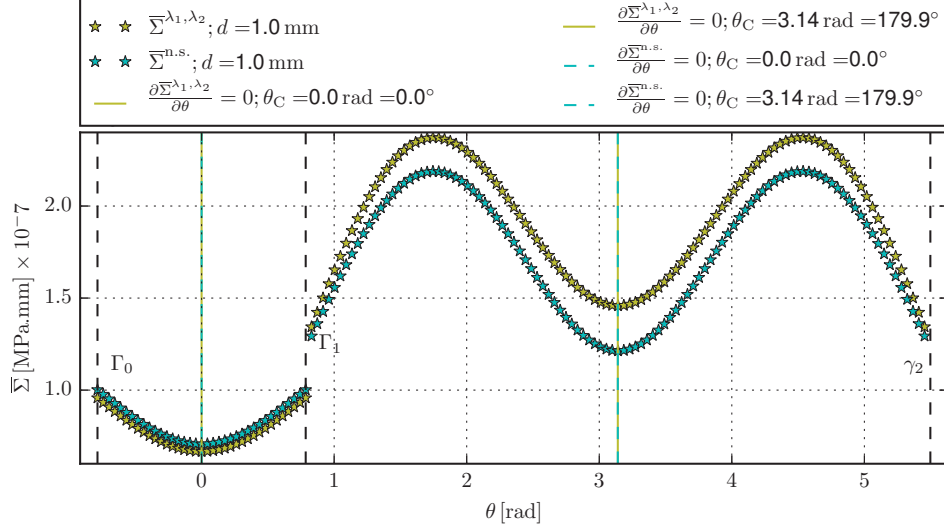
Figure 13: Average value of the \bar{\Sigma}(\theta) plotted by (i) singular terms: the yellow line, by (ii) singular and non-singular terms (the cyan line). The black dashed lines denote the interfaces.
