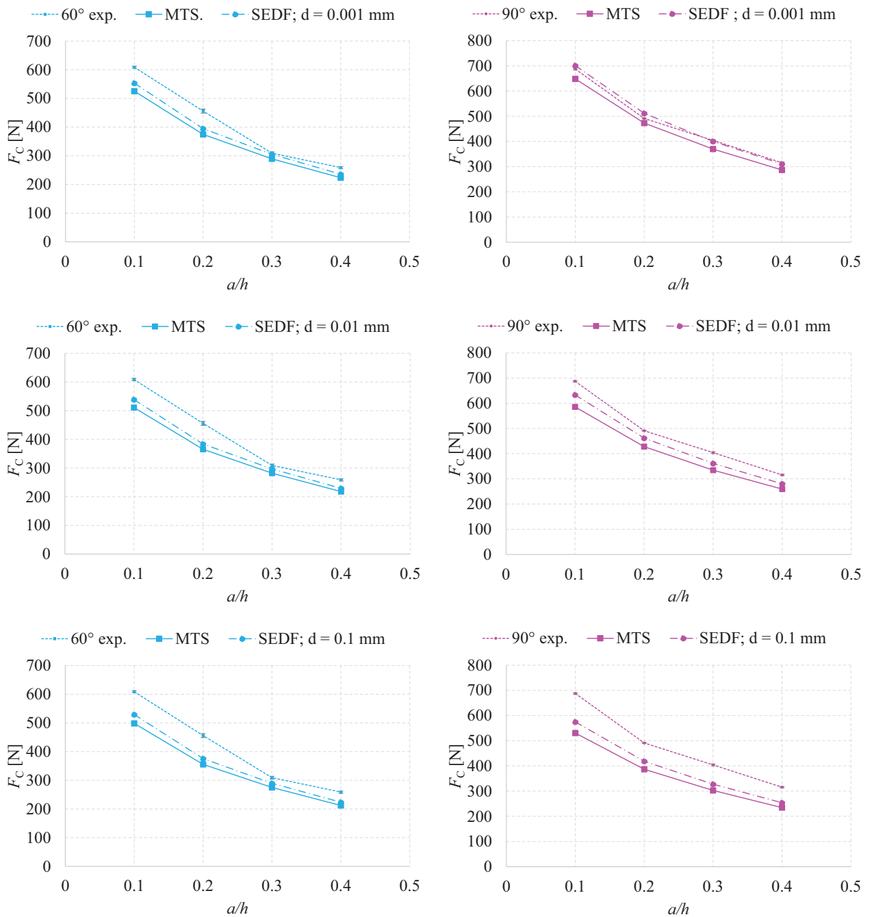
Figure 6: Comparison of experimental failure forces [42], the MTS and SEDF criterion predicted critical forces for a V-notch. The cyan color represents results of 2\alpha = 60^\circ and the magenta color represents results of 2\alpha = 90^\circ .
