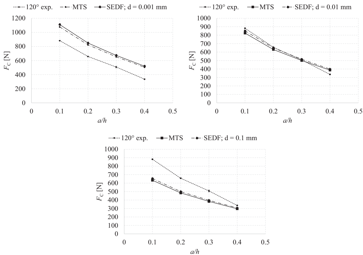
Figure 7: Comparison of experimental failure forces [42], the MTS and SEDF criterion predicted critical forces for a V-notch. Results of 2\alpha = 120^\circ .
