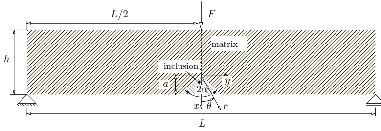
Figure 11: Model of the sharp material inclusion specimen subjected to 3 point bending.
