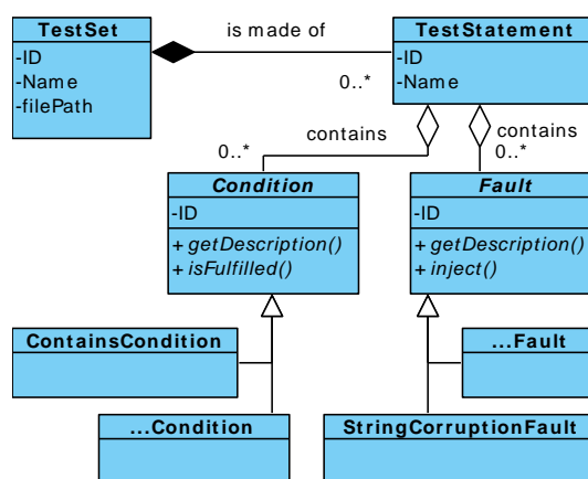
Figure 3: The class diagram of test specifications.
