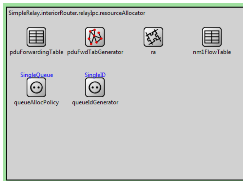
Figure 28. Resource Allocator
