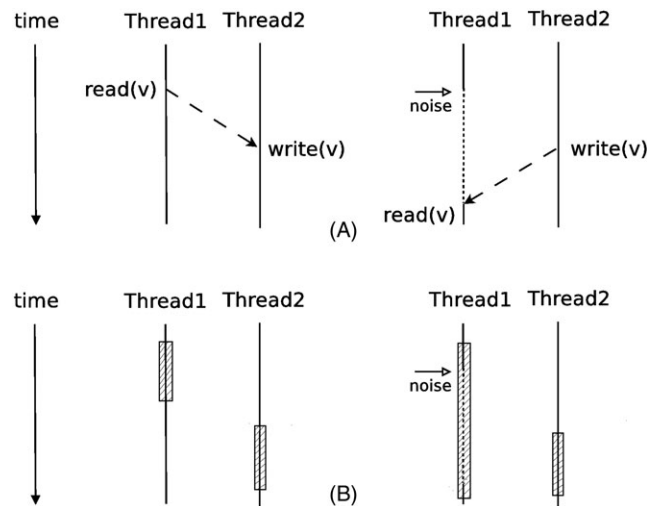
FIGURE 1 Two examples of the effect of noise injection: A, reordering of the common order of two events in a concurrent programme execution and B, prolongation of the time spent by a thread in a critical section, leading to an overlapped execution of two critical sections
